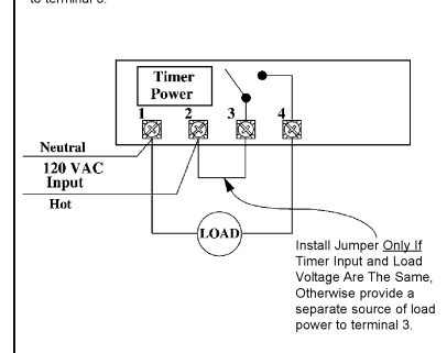
FIG. #3 ET171C SPST
