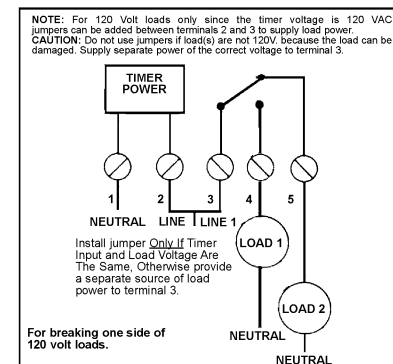
FIG. #5 ET175C SPDT
